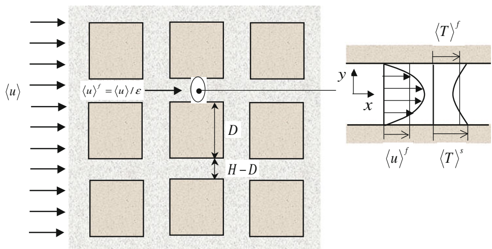
Fig. 2 Model consisting of square tubes for evaluation of the shape factor
